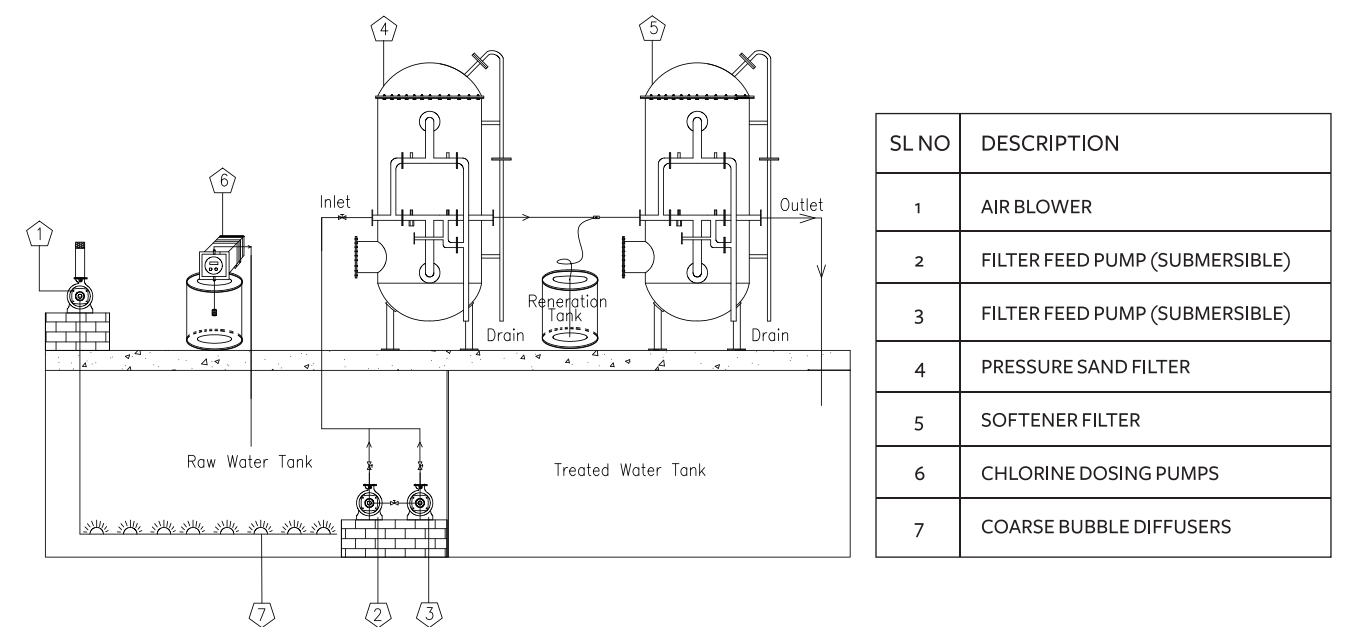
SCHEMATIC DRAWING OF WTP PLANT
