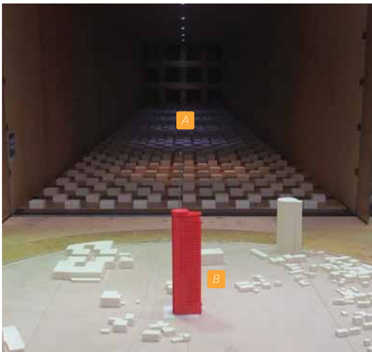
A The wind tunnel tool propelled by powerful fan systems.
